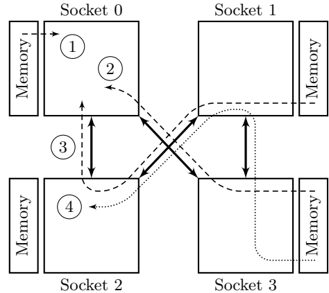
Figure 2: Data access pattern in a 4-socket configuration with 4 QPI links.
