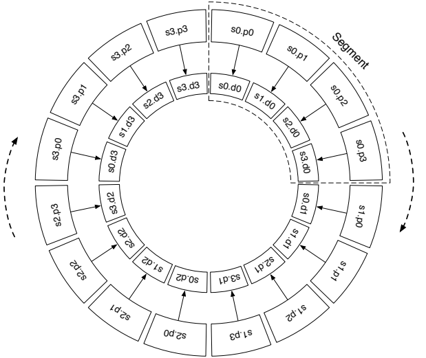
Figure 5: Ring shuffling, an example of a coordinated data shuffling policy.
