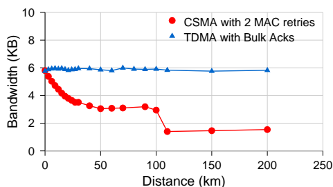
Figure 3: Comparison of WiLD MAC and stock 802.11 MAC
