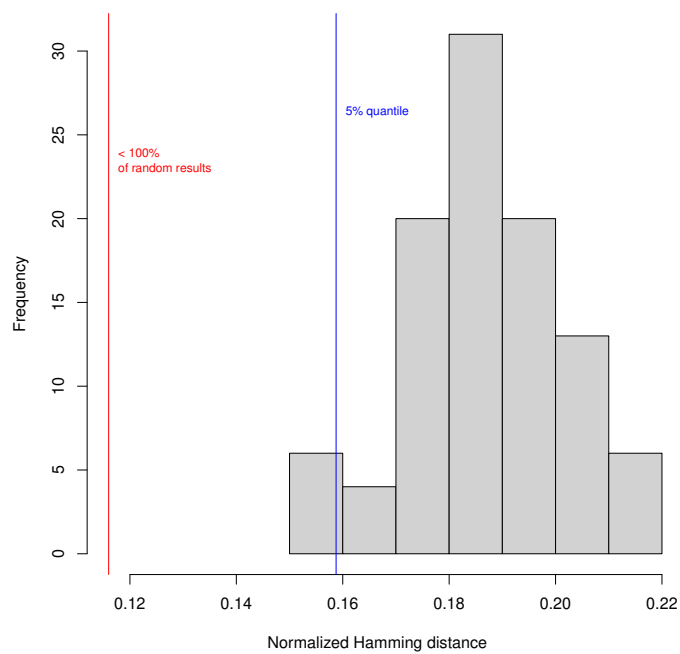
Figure 9: Top: Attractor robustness of randomly generated networks (histogram) in comparison to the mammalian cell cycle network (red line).
