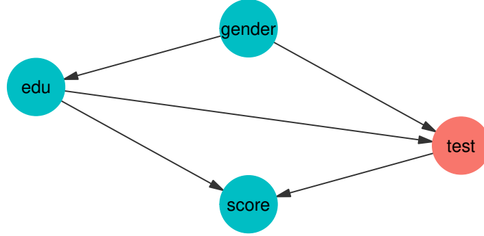
Figure 12: Visualization of the causal graph corresponding to the university admissions example introduced in Section 2 with the variable test chosen as a resolving variable and therefore highlighted in red.
