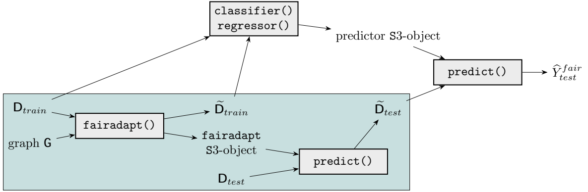
Figure 5: The typical workflow when using fairadapt . The shaded region represents the fair preprocessing which happens within the fairadapt package. Often, this is followed by applying a regressor or a classifier to the transformed data, in order to obtain fair predictions. The latter part is up to the user and not included in fairadapt .
