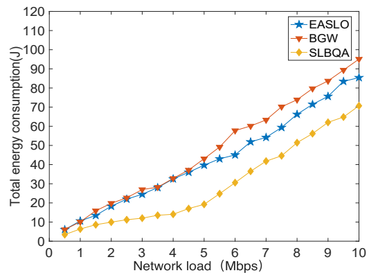
Fig. 4. Total energy consumption with different algorithms
