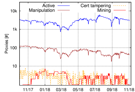
Figure 4. Open proxy ecosystem and miners evolution.
