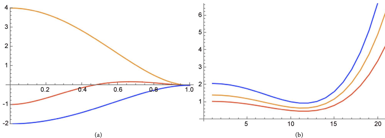
Figure 1. (a) three different choices for f . (b) the graphs of the corresponding functions I(b) .
