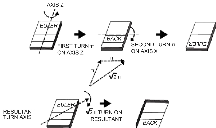
Figure 6. Angular displacement does not obey the law of vector addition [16].
