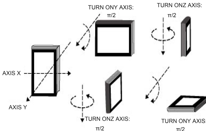
Figure 7. The result of two angular displacements referred to external axes differs depending on the order of application. The end position of the book is different after applying a quarter rotation on two different axes at different successive times [18].
