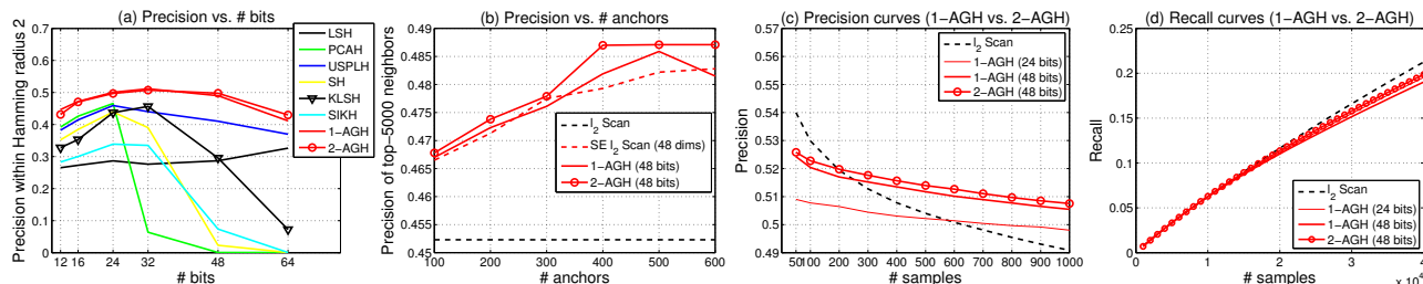
Figure 3. Results on NUS-WIDE . (a) Hash lookup precision within Hamming radius 2 using the varying number of hash bits ( r ); (b) Hamming ranking precision of top-5000 ranked neighbors using the varying number of anchors ( m ); (c) Hamming ranking precision curves; (d) Hamming ranking recall curves.
