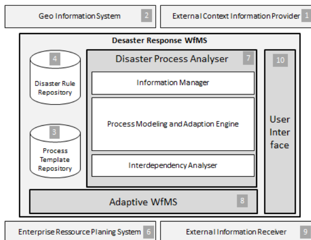
Figure 1. Integrated architecture for DRWfMS
