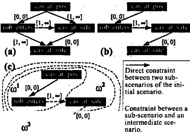
Figure 3. To compile the scenario "Bank attack", we build: (a) the graph with all temporal constraints K^T(\Omega) , (b) the simplified graph with only the necessary constraints and (c) the generated intermediate scenario models.
