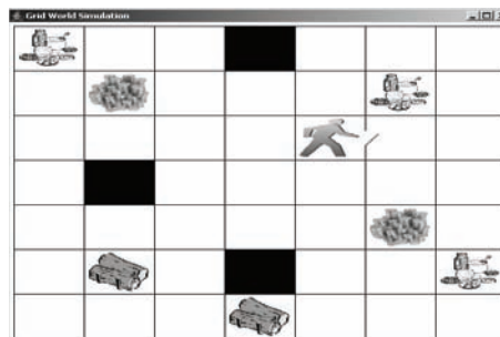
Figure 1: Doorman Domain.
