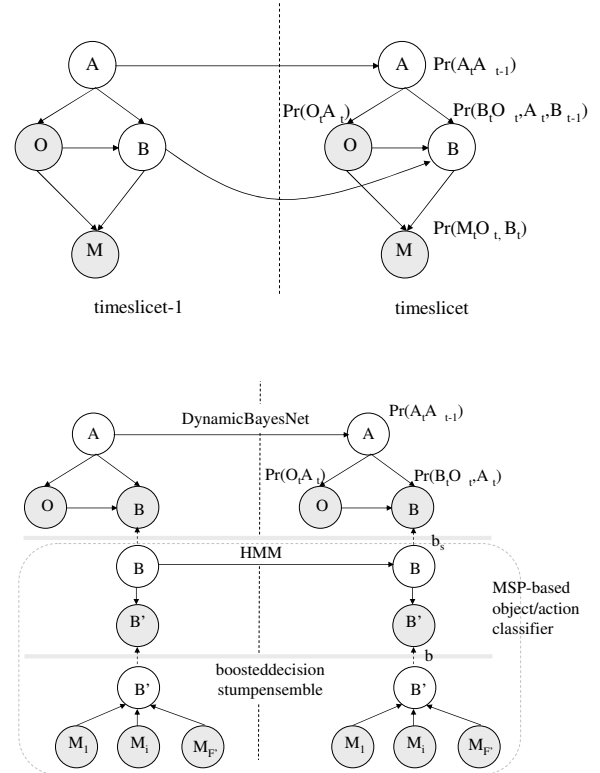
Figure 2: Joint models for activity and action recognition. (a) Full joint DBN (above), and (b) a derived layered model used in this paper (below). Dotted arrows represent the assignment of the MAP estimate of a variable in one layer as its observed value in the next.
