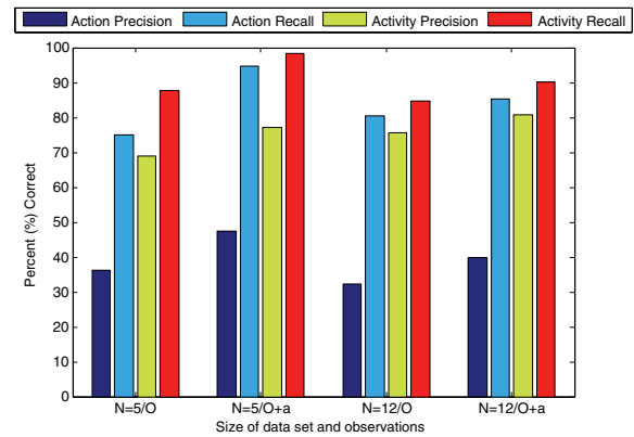
Figure 3: Overall precision/recall
