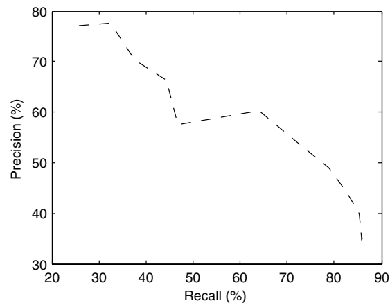
Figure 5: Precision/recall vs. margin threshold
