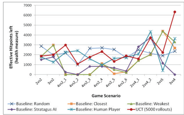
Figure-3: Hit point results for UCT(t) and baselines.
