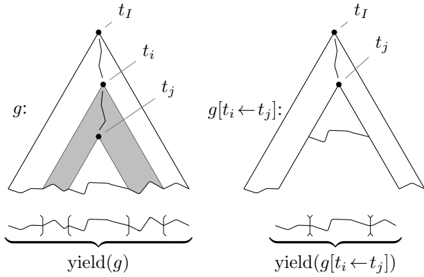
Figure 1: On the left, a decomposition tree g is depicted. The result of the subtree substitution that replaces the subtree below t_i with the subtree below t_j is shown on the right. The gray area inside g corresponds to the tasks that get removed during the substitution. Note how the subtree substitution affects the yield of the tree by removing the contribution of the gray area.
