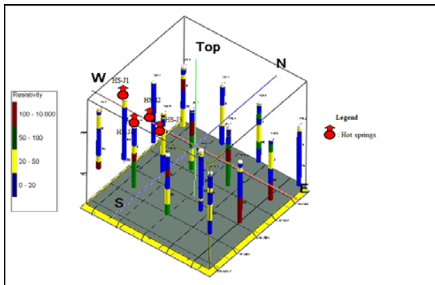
Fig. 4 Results of the interpolation of VES point
