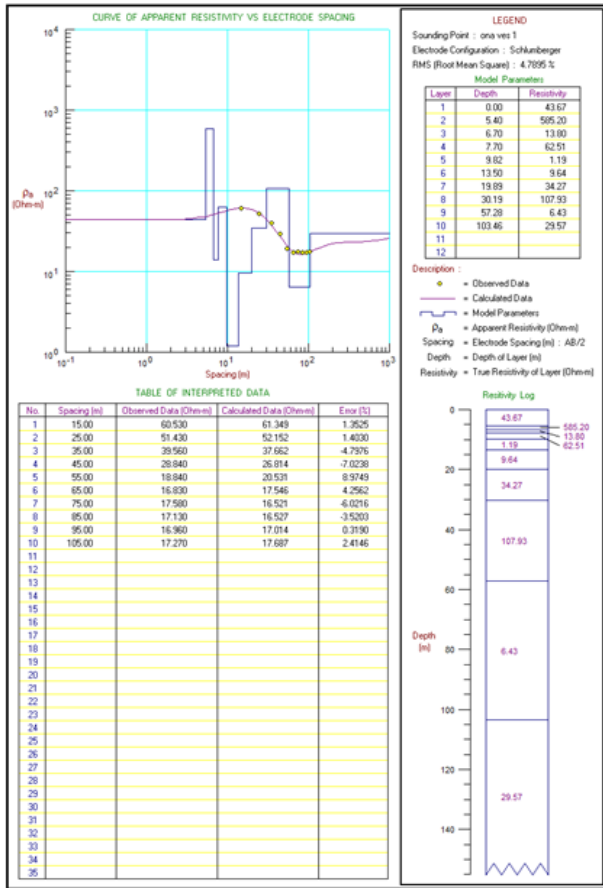
Fig. 3 Results of ID inversion at VES points
