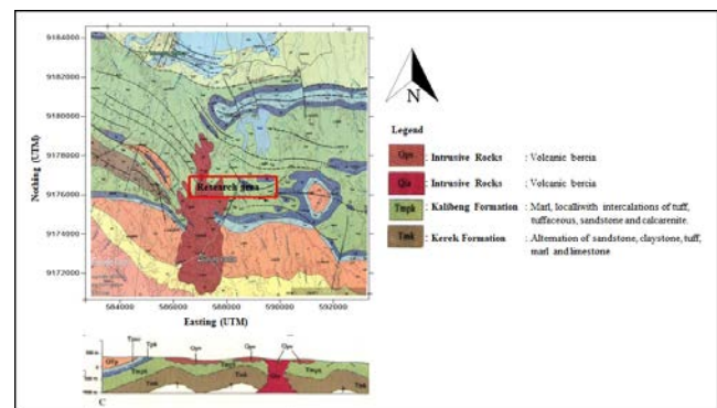
Fig. 1 Geological Map of Bojonegoro Region [2]
