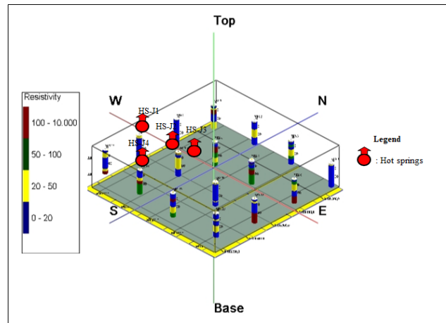
Fig. 5 3D modeling of VES data
