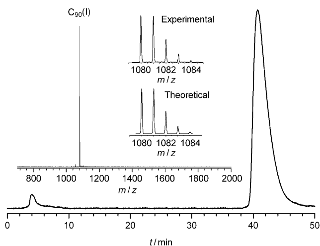
Figure 1. HPLC profile of C_{90} (I) on a Buckyprep column ( 10 \times 250 \text{ mm}^2 ) with toluene as the eluent ( 4.0 \text{ mL min}^{-1} ). The inset shows the LD-TOF mass spectrum and expansions of the experimental and theoretical isotope distributions for C_{90} (I).
