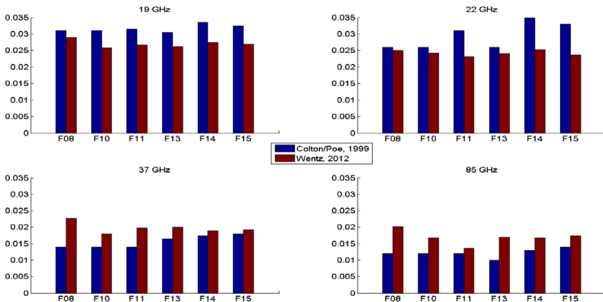
Figure 2. A comparison of the spillover \eta values obtained from pre-launch antenna range measurements [Colton and Poe, 1999] versus the values derived herein using the ocean RTM as the absolute calibration reference.
