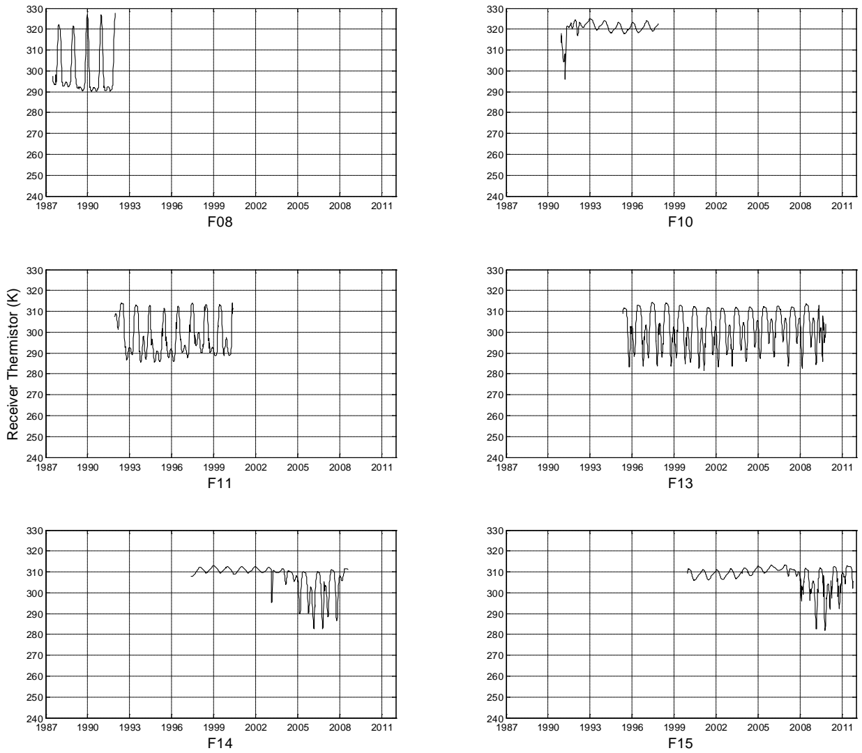
Figure 3A. Same as Figures 1A and 2A except the thermistor is on the internal electronics. Note the anomalously high temperature for the F10 SSM/I. This high temperature may be responsible for F10's unusual calibration problems (see Section 9).
