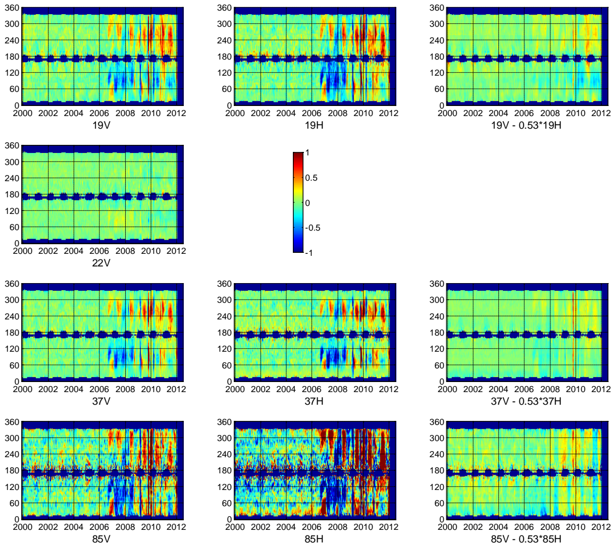
Figure 11. The F15 SSM/I closure residual \delta T_{A,closure} (K) plotted versus spacecraft orbit position \psi (y axis) and time (x-axis) for v-pol (first column), h-pol (second column), and the linear combination V-0.53H (third column), which is insensitive to atmospheric variations. The color bar goes from -1 K to +1 K. In August 2006, the RAD-CAL beacon was turned on, and at this point the closure residuals become large.
