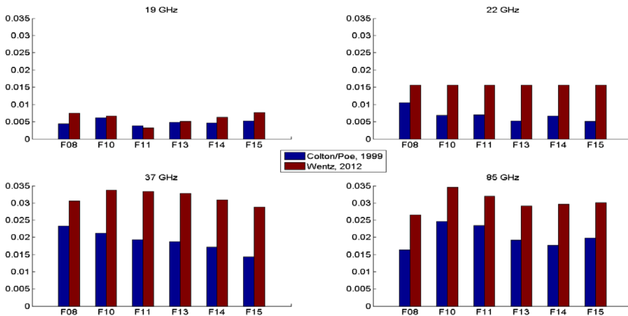
Figure 3. A comparison of the polarization coupling \chi values obtained from pre-launch antenna range measurements [Colton and Poe, 1999] versus the values derived herein using the ocean RTM as the absolute calibration reference. The pre-launch values are systematically lower than those derived from the RTM. Other MW sensors like WindSat show better \chi agreement with the RTM.
