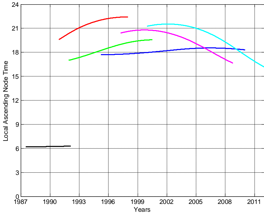
Figure 1. Local time for the ascending node. Each SSM/I is shown in a different color.
