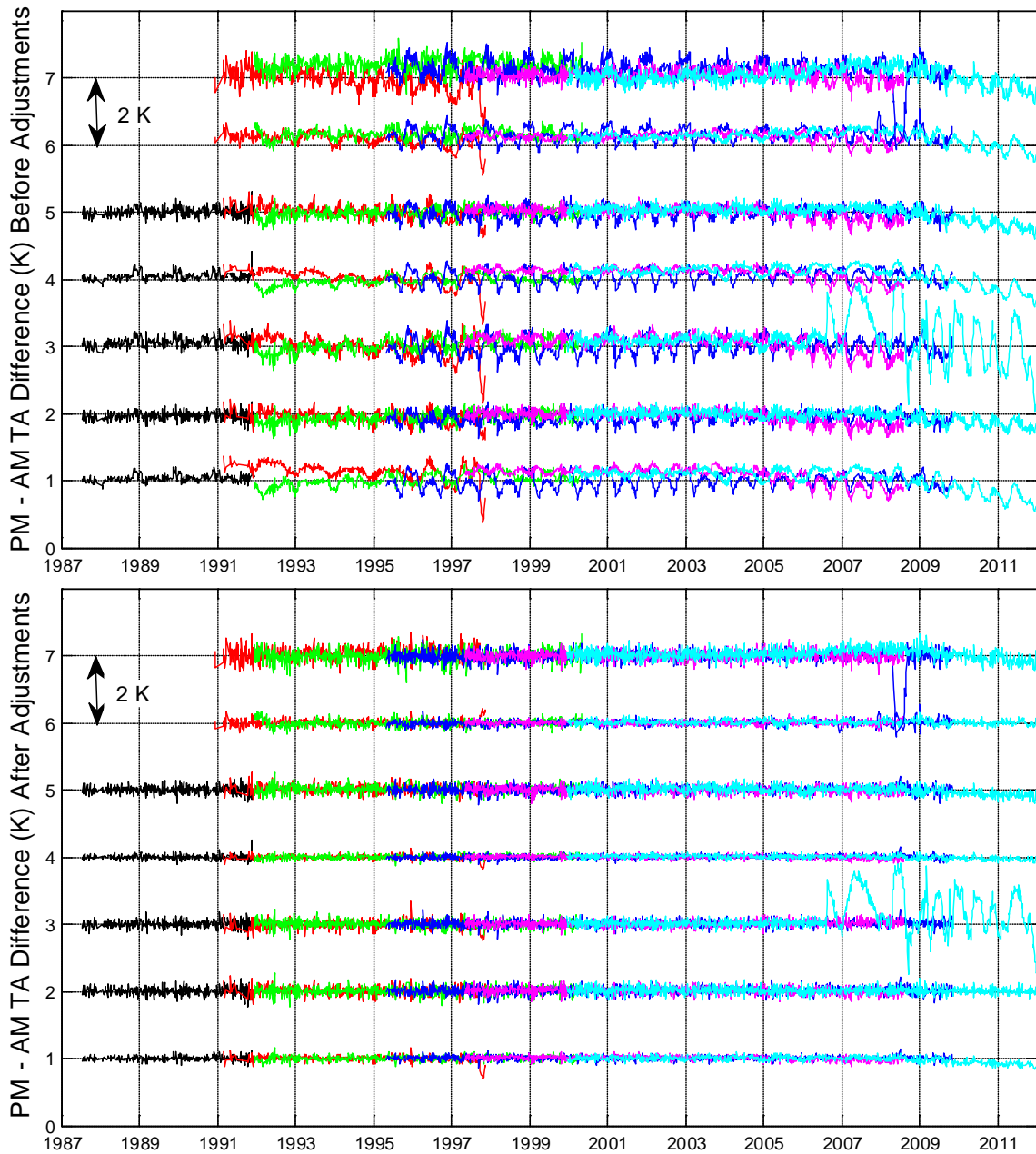
Figure 16. The pm minus am T_A difference for the 6 SSM/I's, with each SSM/I shown in a different color as indicated in Table 6. The top (bottom) frame shows the results before (after) applying adjustments. The labels on the vertical axis denote channel number (1=19V through 7=85H). The vertical scale for the T_A differences is such that 2 K corresponds to the distance between the channel zero lines. The 22V channel for the F15 SSM/I (cyan curve) shows residual errors due to the RADCAL beacon that turned on in August 2006. Also, the 85H channel for the F13 SSM/I (blue curve) shows an unexplained anomaly in 2008. Otherwise, the adjusted results show good pm versus am agreement.
