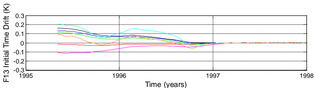
Figure 12. Early mission time drift \Delta T_{A,drift} for the F13 SSM/I. The 7 colors correspond to the 7 channels as indicated in Table 6.
