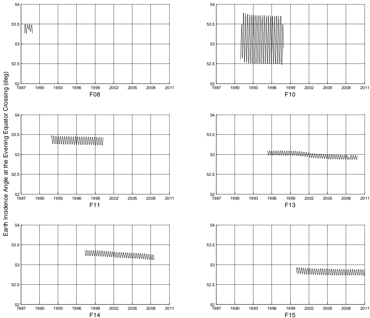
Figure 4A. Mission-long time series of the Earth incidence angle \theta_i at the point of the evening equator crossing. All SSM/Is exhibit an \theta_i oscillation with a period near 120 day. This is due to a combination of the elliptical orbit, the oblate Earth, and the precession of perigee. Due to a malfunction in the launch of F10, the spacecraft did not end up in the desired orbit. Its orbit was more elliptical than the other SSM/Is, and this is why the amplitude of the \theta_i oscillation is so much larger. This large \theta_i oscillation for F10 provides an excellent testbed for verifying the RTM \theta_i functionality (see Section 9).
