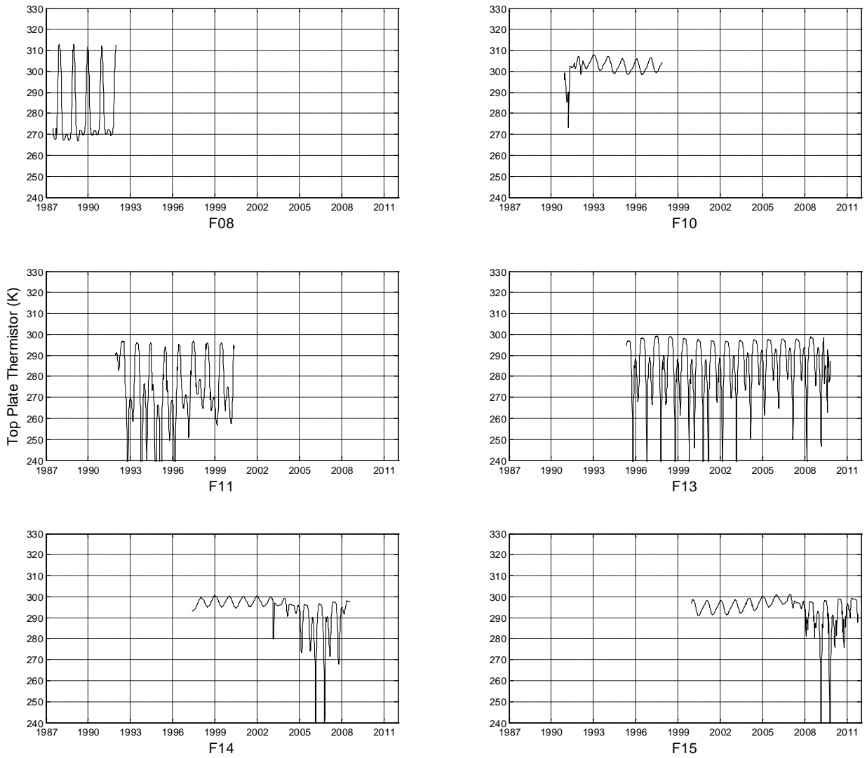
Figure 2A. Same as Figure 1A except the thermistor is on the top of SSM/I ‘drum’ that faces the hot target. These time series are very similar to Figure 1A because both temperatures are external readings in close proximity.
