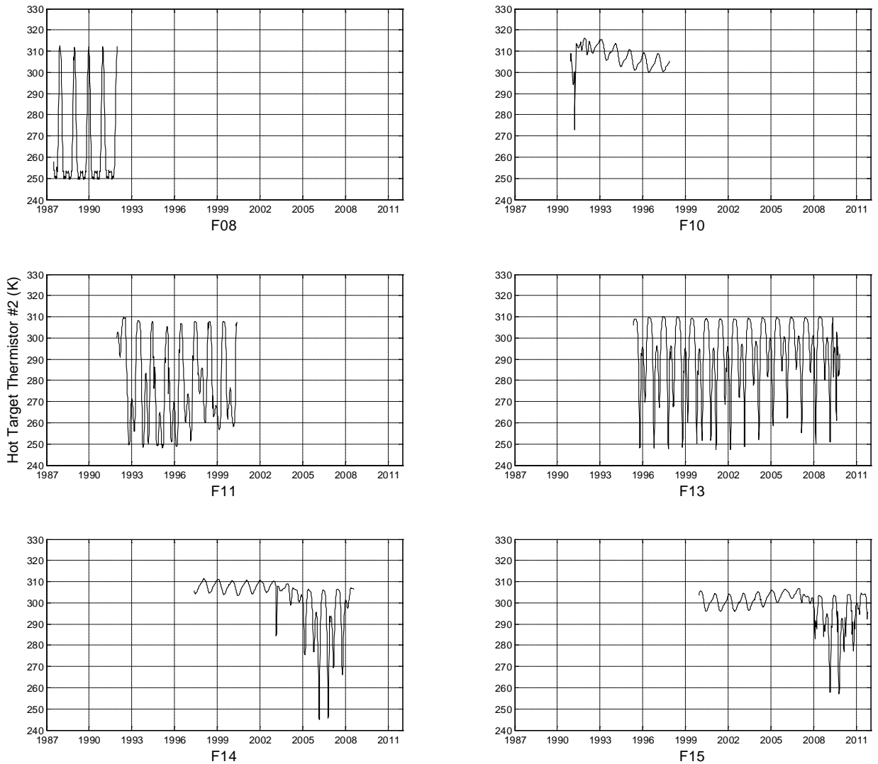
Figure 1A. Mission-long time series of hot target thermistor #2. Global, pentad-averaged values are shown. The other two hot target temperatures are essentially the same when shown at this scaling. When the satellite's equator crossing is in the early morning/evening ( \approx 6 am and 6 pm), the hot target temperature experiences a large seasonal variation as compared to the late morning/evening for which there is little seasonal variation. See Figure 1 for equator crossing times.
