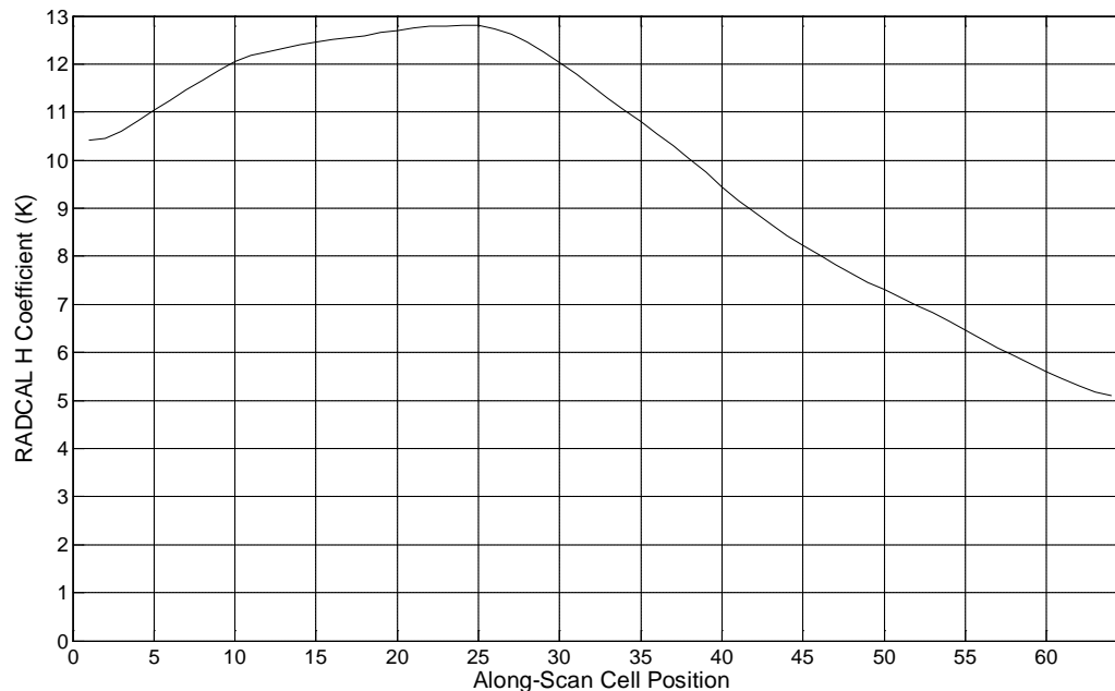
Figure 10. The RADCAL H_1(\omega) function plotted versus scan position.
