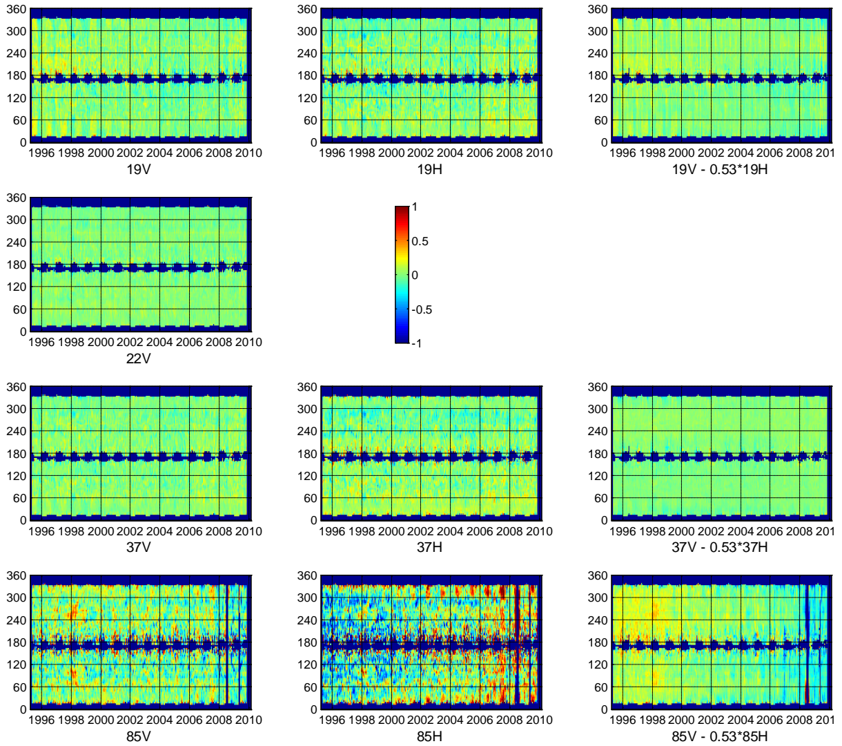
Figure 6. The F13 SSM/I closure residual \delta T_{A, \text{closure}} (K) plotted versus spacecraft orbit position \psi (y axis) and time (x-axis) for v-pol (first column), h-pol (second column), and the linear combination V-0.53H (third column), which is insensitive to atmospheric variations. The color bar goes from -1 K to +1 K.
