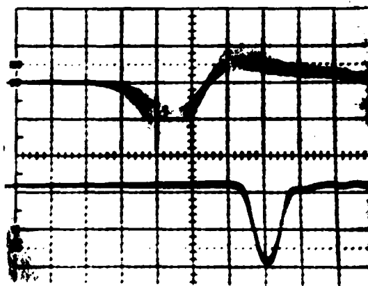
FIG. 3 - (top) Typical photomultiplier signals from a ^{90}\text{Sr} source (20mV/div, 2 ns/div); (bottom) Zero crossing discriminator output signals (500mV/div, 2 ns/div). The oscilloscope is triggered on the zero crossing output signal).
