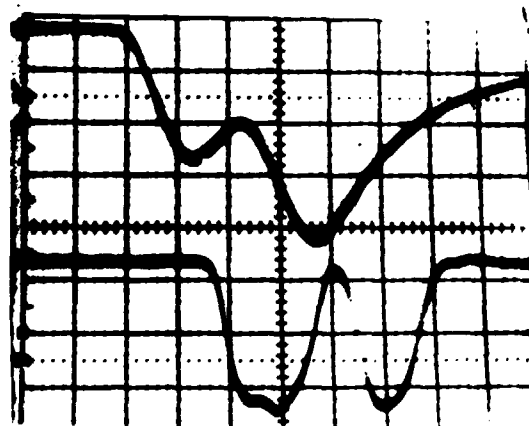
FIG. 4 - (top) Two "splitter" output signals separated by 5 ns after 90 m of RG58 cable (100 mV/div, 2 ns/div); (bottom) Trigger receivers output signals (500 mV/div, 2 ns/div).
