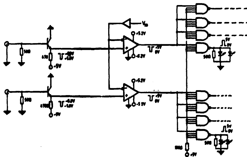
FIG. 5 - LED's driving circuit.
