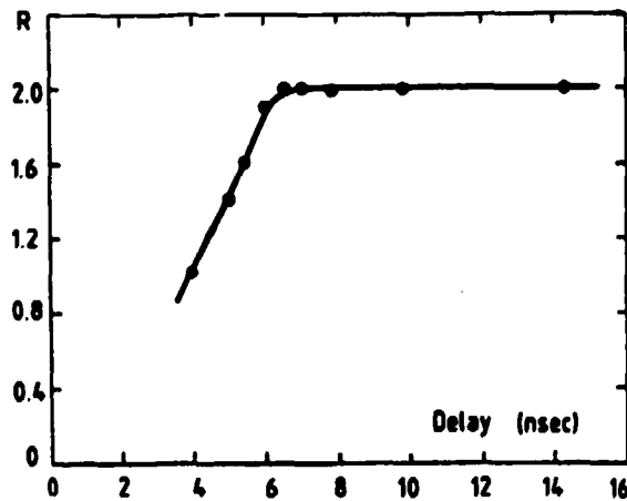
FIG. 8 - Double pulse resolution including the photomultiplier and the LED driving system.
