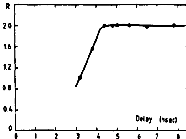
FIG. 9 - Double pulse resolution due to electronics only with a simulated input pulse.
