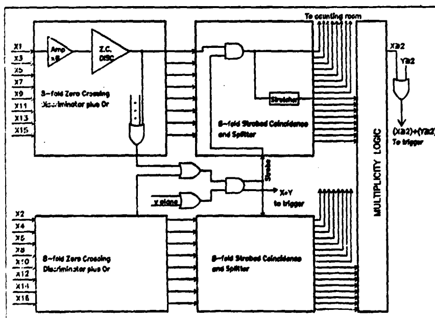
FIG. 2 - Block diagram of the close electronics.
