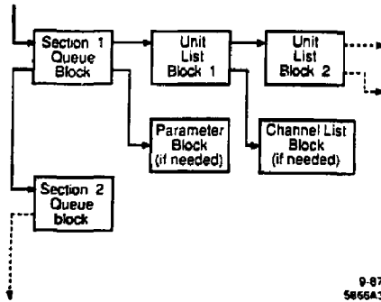
Fig. 3. Section and unit list queue.
