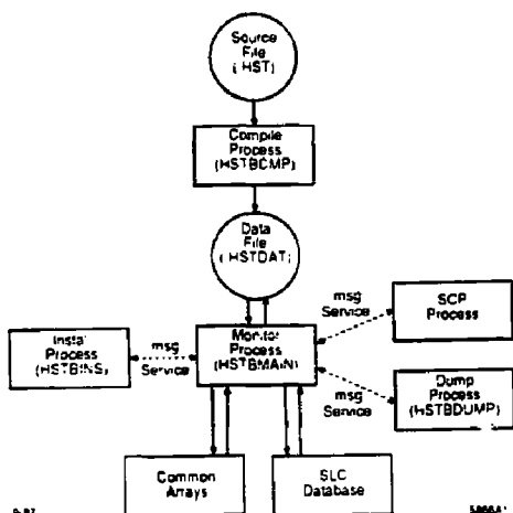
Fig. 1. History data system.
