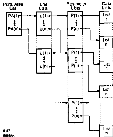
Fig. 4. Internal database Index structure.
