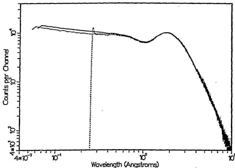
Figure 1. Beam monitor raw data (not corrected for efficiency) measured on the H1 beamline at IPNS using a \text{BF}_3 ionization chamber. Dashed line - original preamplifier/amplifier; Solid line - new bipolar preamplifier/amplifier; Dotted line - same new preamplifier and same detector, but in a location further downstream where the incident intensity was attenuated by a factor of 6. All were arbitrarily scaled to match at the Maxwellian peak. Note that with the old preamplifier the detector was effectively "dead" for wavelengths below \sim 0.25 \text{ \AA} and the spectrum was somewhat distorted for wavelengths just above this. The small discrepancies at short wavelengths between the two measurements with the new preamplifier/amplifier are not yet fully understood and may represent real spectral differences at the two beam locations. Small differences at the longer wavelengths are due to differing numbers of Al windows upstream from the detector.
