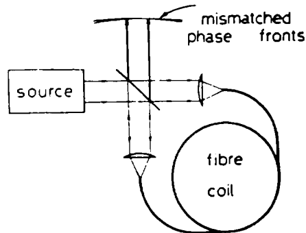
Fig. 7 Ring interferometer with a multiturn fiber coil.
