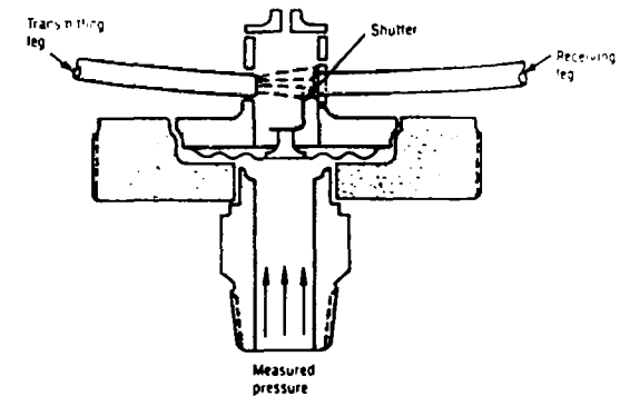
Figure 5 Transmissive Fiber Optic Pressure Sensor Using a Shutter to Modulate the Intensity
