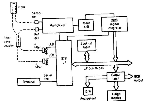
Figure 4 Sensor System Schematic
