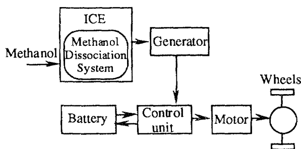
Figure 2. Scheme of the series hybrid propulsion system with on-board methanol dissociation
