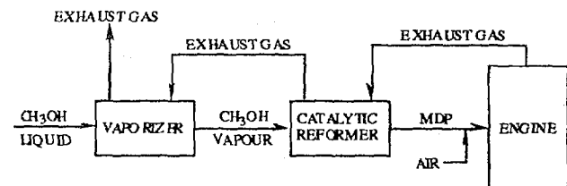
Figure 1. Scheme of on-board methanol dissociation system (based on [8])
