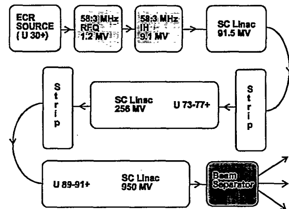
Figure 1: Elements of the proposed linac
