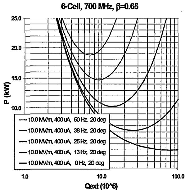
Figure 4: RF power required for phase control in the presence of microphonic frequency noise.
