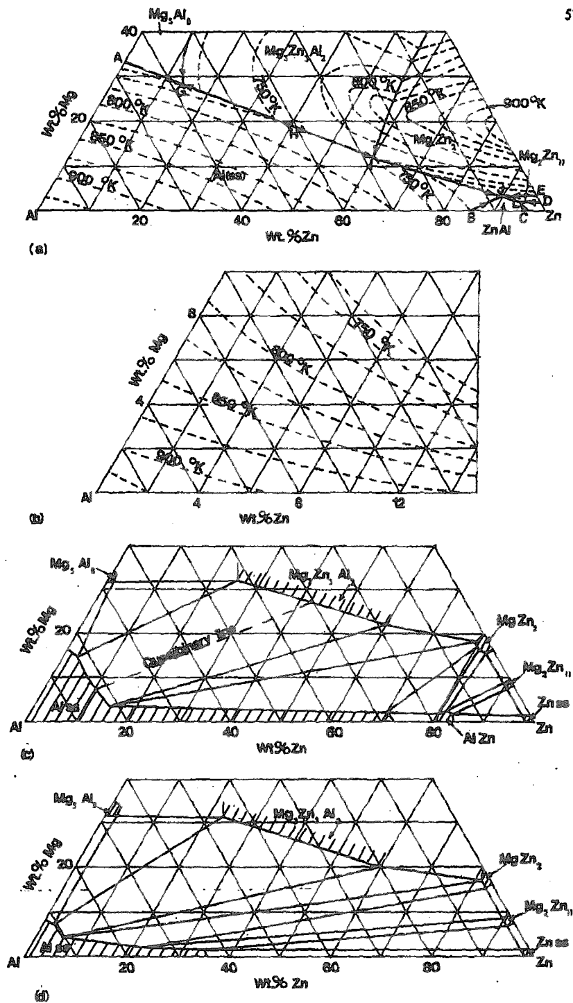
Figure 3.46. Aluminum-zinc side of the aluminum-magnesium-zinc equilibrium diagram: (a) liquidus; (b) solidus; (c) phase distribution just below the freezing point; (d) phase distribution at 500°K
