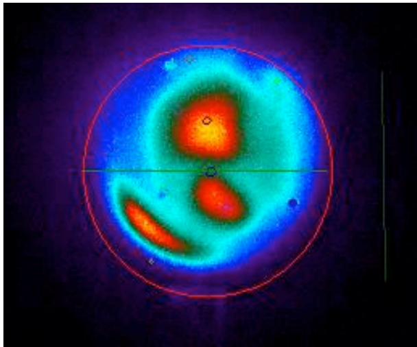
Figure 6: IR camera data from target of a high density helicon plasma showing azimuthal asymmetries in heat flux pattern.
