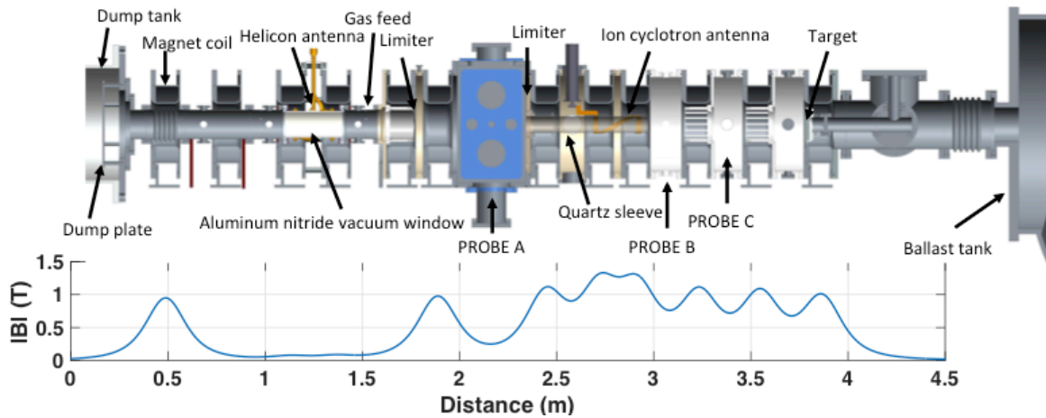
Figure 3: Proto-MPEX: Magnet coils are counted from left to right (From 1 to 12). Vacuum chambers in between coils are labelled as: 6.5 for vacuum chamber (spool piece) between coil 6 and 7 for example.
