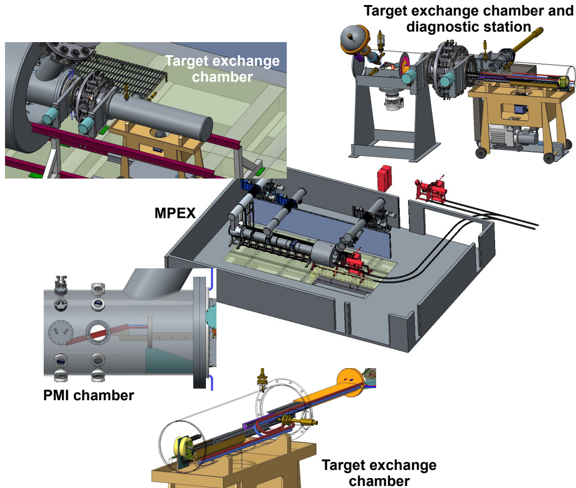
Figure 2: Concept of MPEX with compact target exchange chamber movable from MPEX to diagnostic station to allow for fast evaluation of evolving surfaces.
