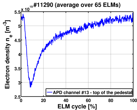
Figure 2: Evolution of electron density on top of the pedestal during the ELM cycle measured by Li-BES
