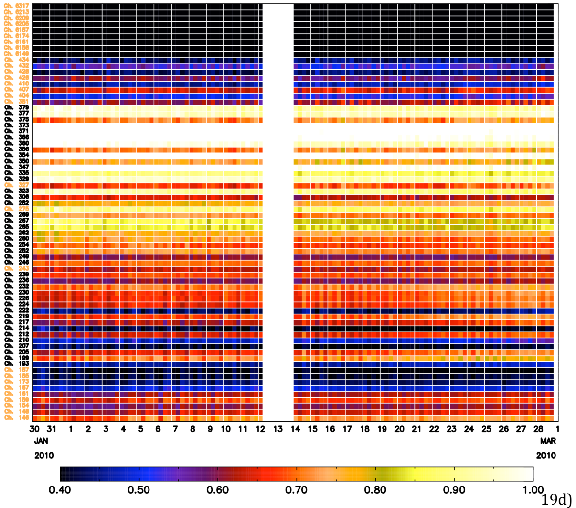
Figure 19: The global 6-hourly standard deviation of the innovations for a selection of IASI channels. Time is along the x-axis, and the IASI channels are along the y-axis with assimilated channels in black. The ‘base’ configuration is in panels 19a and 19c, while the ‘uwemis’ configuration is in panels 19b and 19d.
