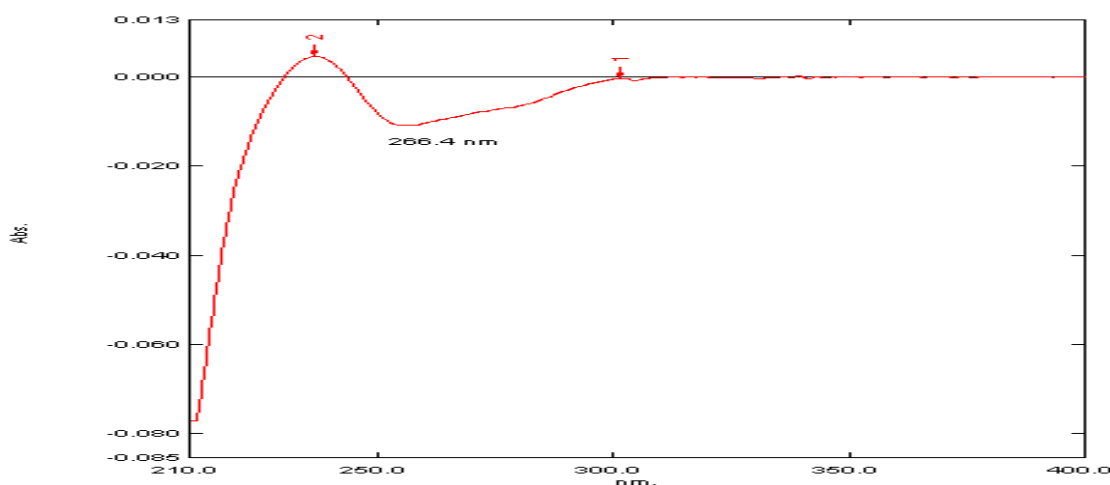
Fig. 3: First order derivative spectra showing peak minima of Teneigliptin
