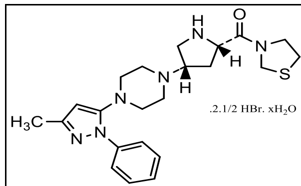
Fig. 1: Teneligliptin Hydrobromide Hydrate Chemical structure
