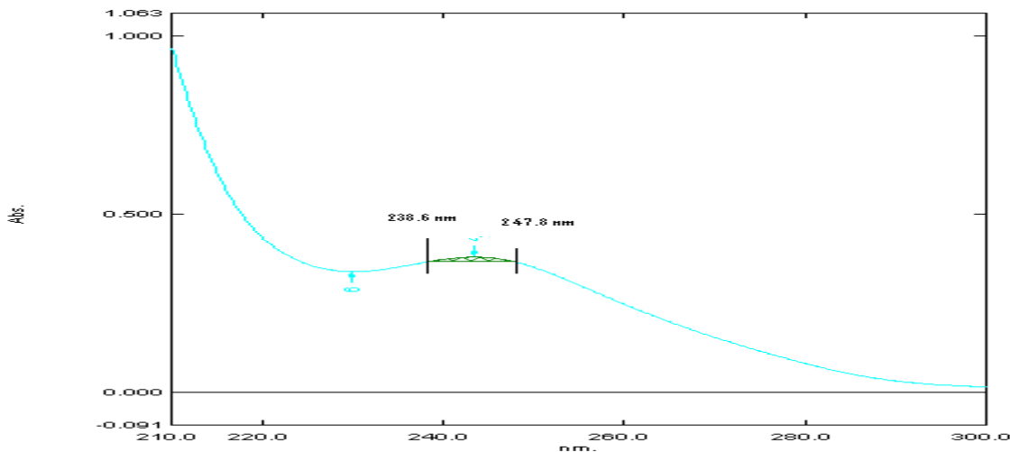
Fig. 4: Area under curve spectra of Teneligliptin
