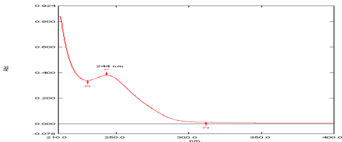
Fig. 2: Zero order spectra showing \lambda_{\text{max}} of Teneigliptin
