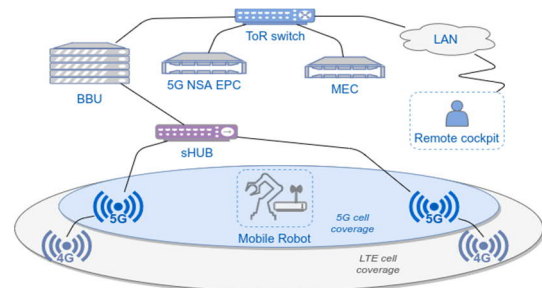
Fig. 3. The high-level 5G network architecture
