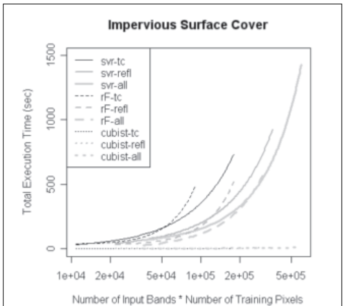
Figure 3. Total execution time to build the estimation model and apply it to the entire study area. Execution time was smoothed using a 2 nd order polynomial fit. The longest RF runs were omitted due to processing limitations. A color version of this figure is available at the ASPRS website: www.asprs.org .
