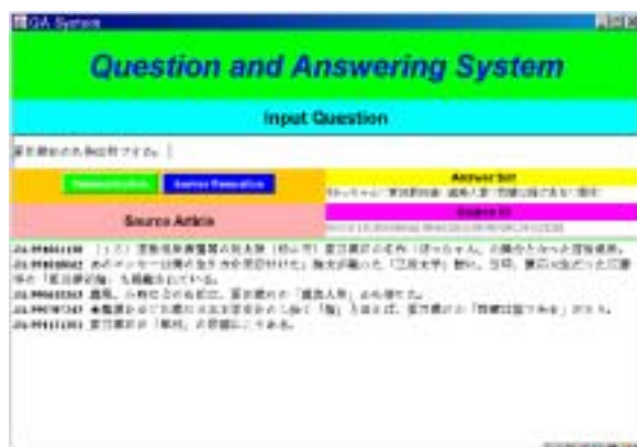
Figure 2. Q&A System
