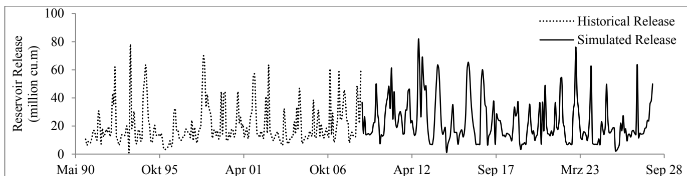
Figure 5. Results of simulated operation using the ANFIS model (20 years simulation period)
