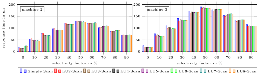
Fig. 4. Response time of branching scans with different unrolling depths for varying selectivities for 30 million data items (LU n = n -times loop-unrolled).
