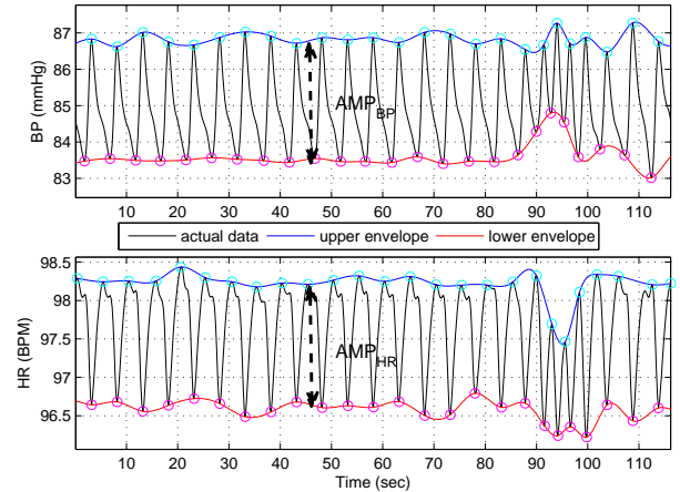
Figure 1. Extracting the upper and lower envelopes of the model outputs, giving rise to the amplitude signals Amp_n^{mo}(t) employed in eqn. (10) for the estimation of respiratory parameters. Top: BP signal. Bottom: HR signal. The synthesized data amplitudes Amp_n^{syn}(t) are computed in the same way.
