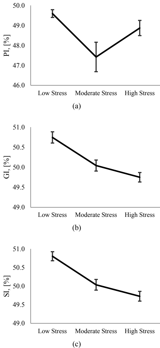
Figure 1. Porta Index (PI), Guzik Index (GI), and Slope Index (SI) across groups with different stress level (the bars show the standard error).
