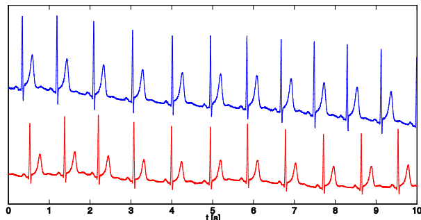
Figure 2. Comparison of the V6 lead acquired (not simultaneously) on the same subject using textile electrodes (top) and Ag/AgCl ones (bottom).
