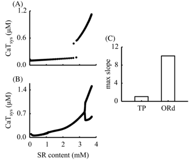
Figure 3. CaT-SR content curve for the TP model (A) and the ORd model (B); Maximum slopes of the CaT-SR content curve of the two models (C).
