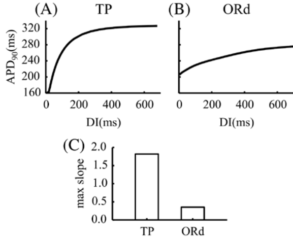
Figure 2. APD restitution curve for the TP model (A) and the ORd model (B); Maximum slopes of the APD restitution curve of the two models (C).
