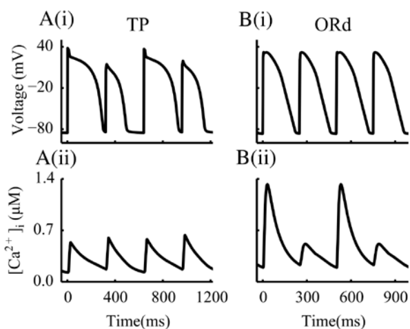
Figure 1. Simultaneously recorded APs (A(i)) and CaTs (A(ii)) at BCL=320ms for TP model; Simultaneously recorded APs (B(i)) and CaTs (B(ii)) at BCL=250ms for ORd model.
