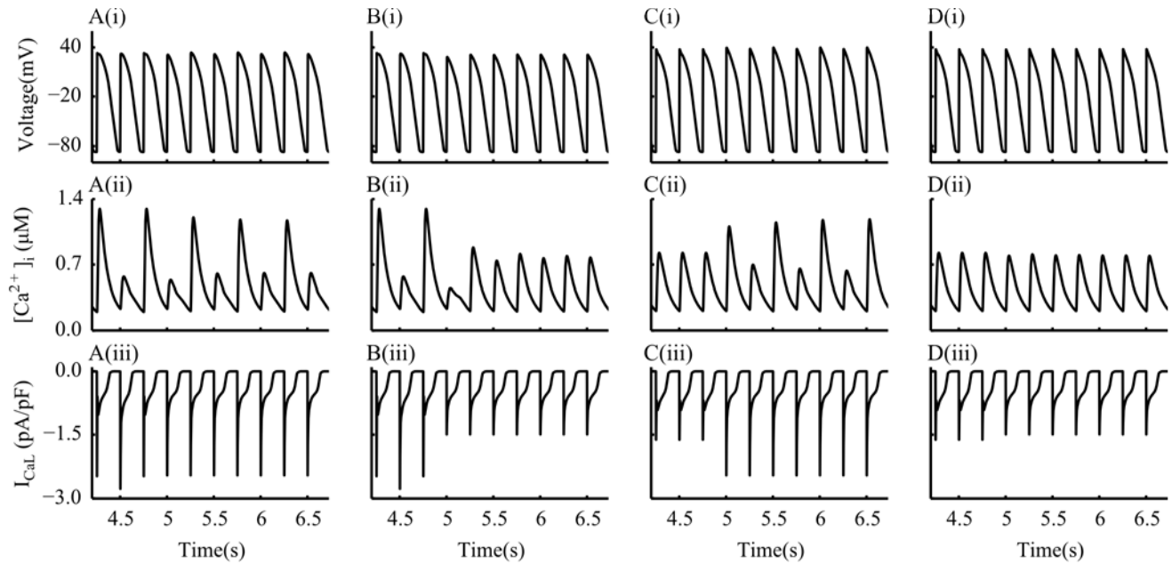
Figure 4. AP (A(i)-D(i)), CaT (A(ii)-D(ii)) and I_{CaL} (A(iii)-D(iii)) time traces for I_{CaL} clamp simulation results: (A(i-iii)) alter system clamped by I_{CaL\_alter} ; (B(i-iii)) alter system clamped by I_{CaL\_normal} ; (C(i-iii)) non-alter system alternans clamped by I_{CaL\_alter} ; (D(i-iii)) non-alter system clamped by I_{CaL\_normal} .
