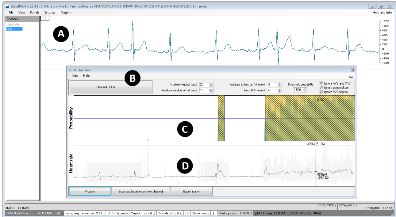
Figure 2. Software implementation of the presented model as a plugin for free SignalPlant [10] software (A). 1-hour ECG was loaded into SignalPlant; only 8 seconds of the signal is displayed. After processing, the plugin window (B) shows two panels: probability in time (C) and heart rate (D). The probability panel shows episodes of atrial fibrillation during the whole recording as hatched areas. The blue line is a threshold set at 0.5 by default; it can be changed. The heart rate panel (D) shows related BPM (median – black line, min/max – grey background). A click with the pointer in area (D) will show BPM values at a specific time and will also change the window displayed in (A); this allows the user to see the studied signal in detail.
