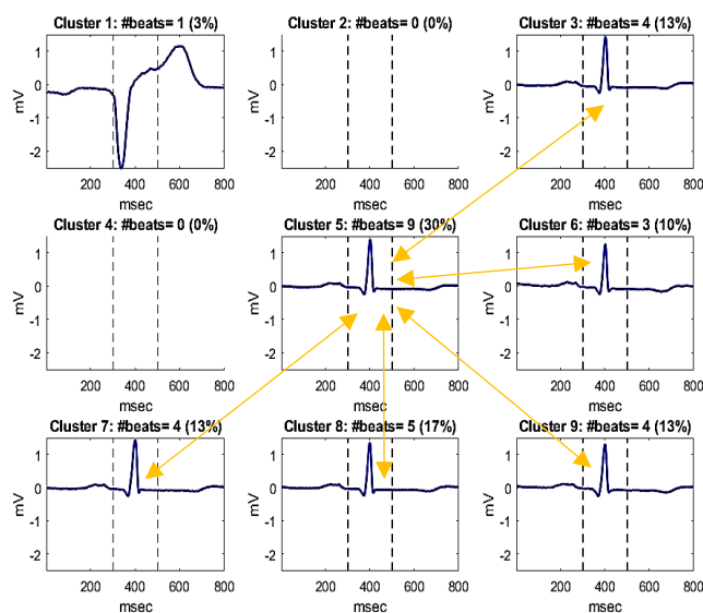
Figure 1. An example of clustering the beats by QRS matching and merging the highly-correlated cluster.
