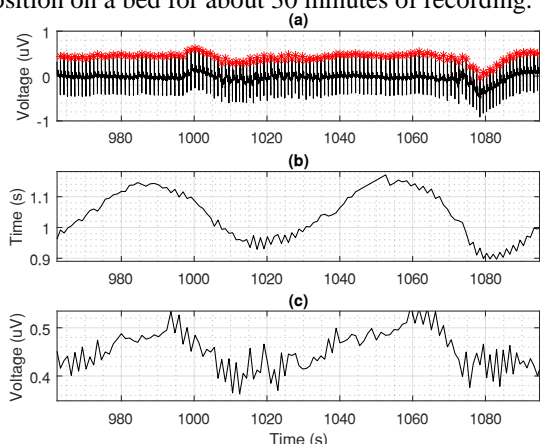
Figure 1. ECG-Derived Respiration construction for the patient n°3 exhibiting a severe Cheyne-Stokes breathing (a) original ECG (lead V3) with annotated peaks (b) Heart-Rate signal (c) R-Wave Amplitude signal.
