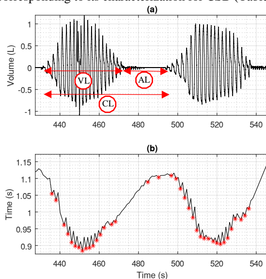
Figure 2. ECG-Derived Respiration for the patient n°3 (severe CSB) (a) Ventilation signal with durations: VL corresponding to Ventilation Length, AL to Apnea Length and CL to Cycle Length (b) Heart-Rate signal with annotated expiration.
