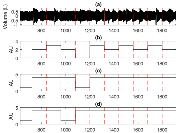
Figure 2. Results of scoring and classification for patient n°2 (a) Ventilation with epochs of 2 minutes (b) Frequential score S_f (c) Respiratory events detected by our method (see Table 3), 9 epochs are classified as CSB hypopneas and 2 epochs as normal breathing, (d) Respiratory events detected by the expert on the ventilation signal, 9 epochs are classified as CSB hypopneas and 2 epochs as normal breathing. 2 epochs are misclassified by our method.
