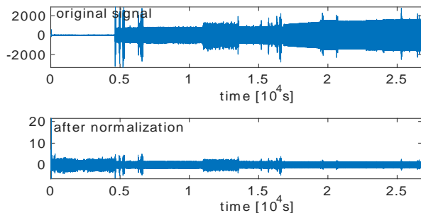
Figure 1. Example of the resulting preprocessing step on an airflow signal
