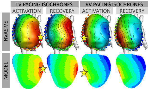
Figure 4. Top: Invasive animal recordings were obtained during pacing on the heart (at the location of the yellow star). Bottom: the computational model was used for virtual pacing at the same location, yielding qualitatively similar patterns of activation and recovery.
