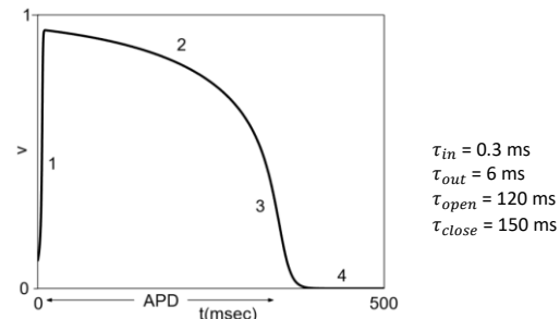
Figure 3. The four phases of the action potential (left) related directly to the four temporal parameters of the Mitchell-Schaeffer model (right). These parameters can be adapted locally to match ECGI findings from an individual patient.
