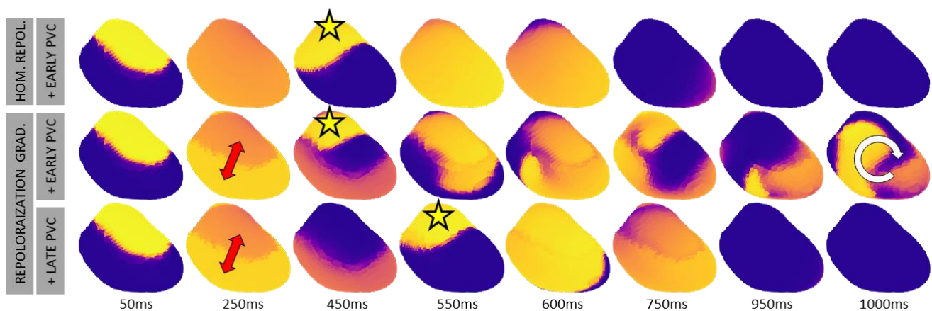
Figure 5. Transmembrane potential maps (blue = resting potential, yellow = peak action potential). Mimicking the observed patient abnormalities, the personalized model shows that re-entry mechanisms (white arrow) only develop in the presence of both the observed recovery gradient (red arrows), and an early premature ventricular complex (PVC, star) as trigger.
