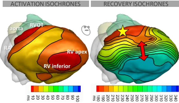
Figure 1. Example of ECGI findings in a patient who had idiopathic VF. Left: Normal activation pattern during sinus rhythm. Right: Abnormally early recovery at the right ventricular outflow tract (RVOT) and steep recovery gradients (arrow). Short-coupled PVCs originated from the RVOT (star).
