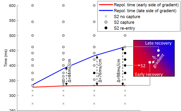
Figure 6. Relationship between the dispersion of recovery times between regions of early (red) and late (blue) recovery, the resulting recovery gradient \Delta , and the inducibility of re-entry when virtually pacing is performed from the S2 location in the early-recovery region. The extra stimulus S2 only results in re-entry when the gradient is large enough (76 or 98 ms/cm) and the timing of S2 is within a small vulnerable window.
