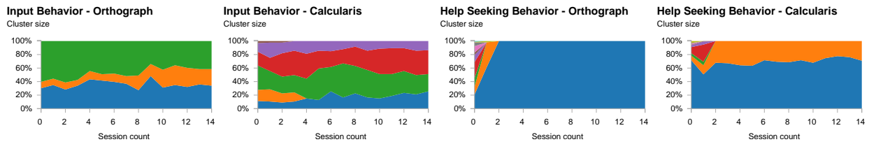
Figure 9: Relative cluster sizes over the first 15 sessions based on the clustering of Input Behavior (left) and Help Seeking Behavior (right) for students training with Orthograph and Calcaris .
