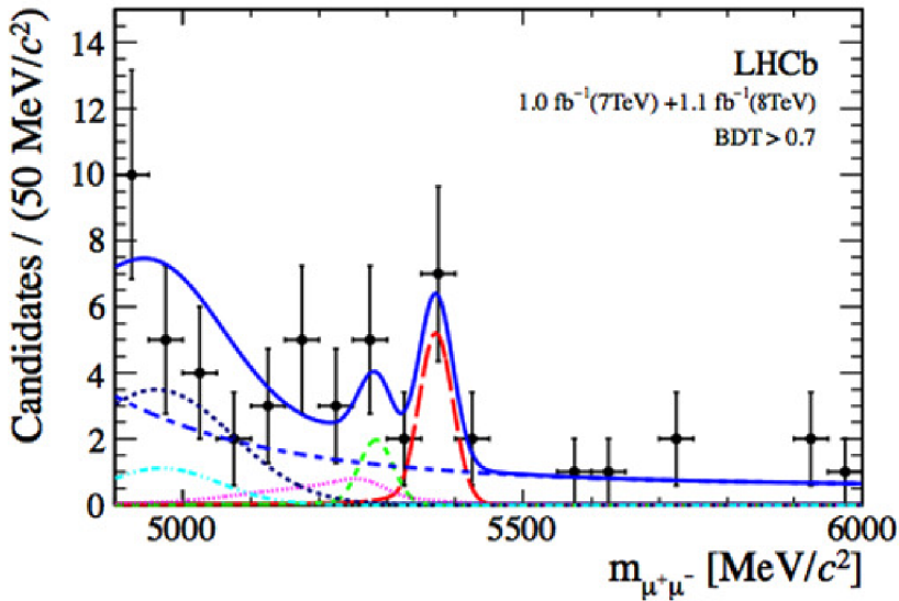
Figure 2. The invariant mass distribution of the \mu\mu system showing the B_s -peak
