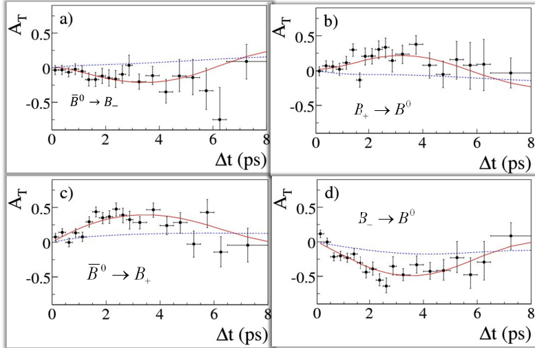
Figure 4. Experimental TRV asymmetries as function of \Delta t
