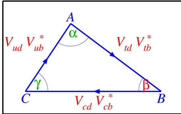
Figure 1. The bd unitarity triangle representing the CKM mixing
