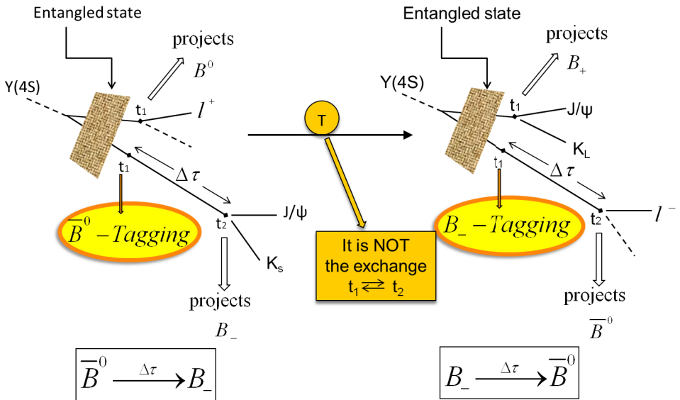
Figure 3. Basic concepts explaining the preparation and detection of initial and final meson states, for the Reference and T-reverse transitions, by means of the experimental time-ordered decay channels to definite flavour and CP eigenstates.
