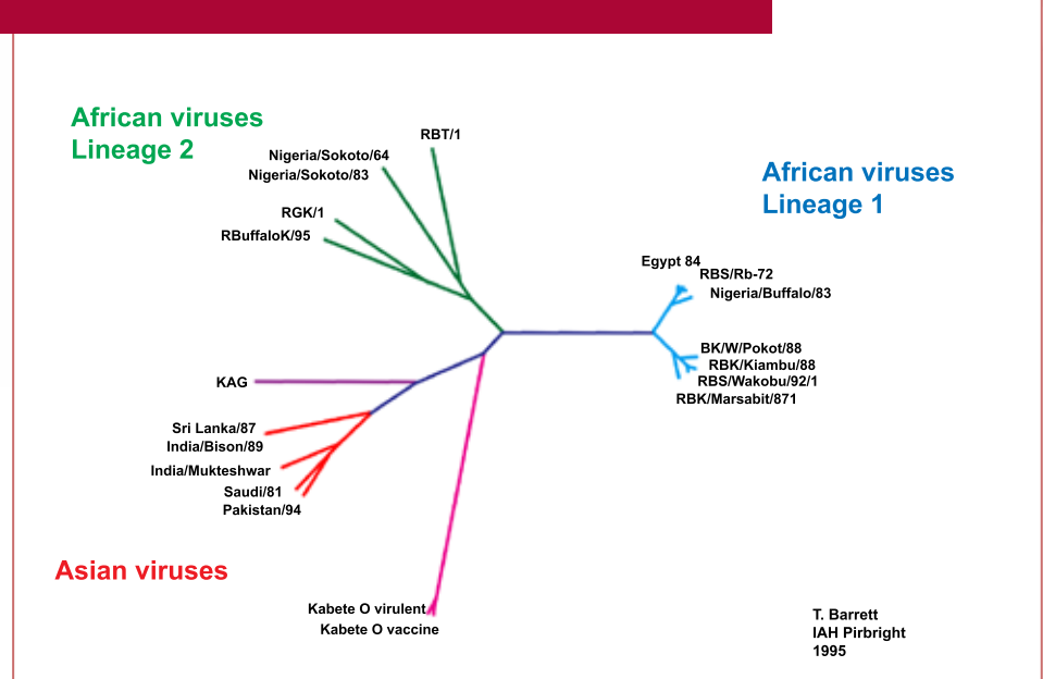
Figure 1: Phylogenetic relationships of rinderpest viruses
