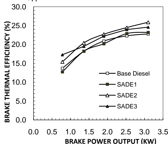
Figure 1. Comparison of brake thermal efficiency with power output for three SADE configurations
