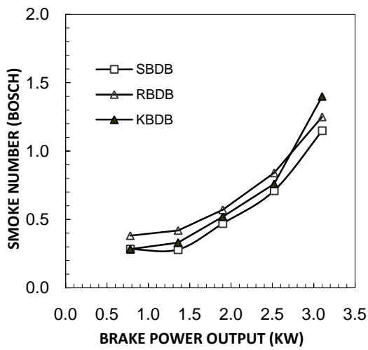
Figure 4. Comparison of smoke number with power output for different Biodiesel blends
