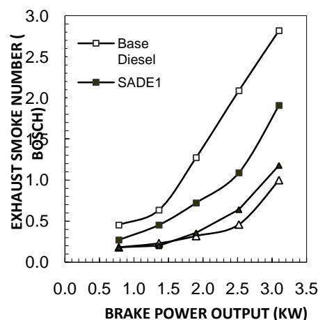
Figure 2. Comparison of smoke emissions with power output for three SADE configurations
