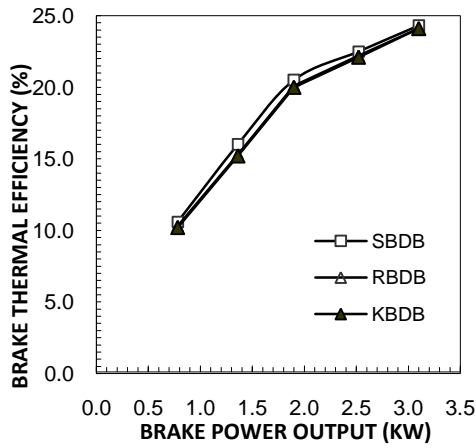
Figure 3. Comparison of brake thermal efficiency with power output for different Biodiesel blends
