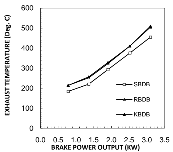
Figure 6. Comparison of exhaust temperature with power output for different Biodiesel blends
