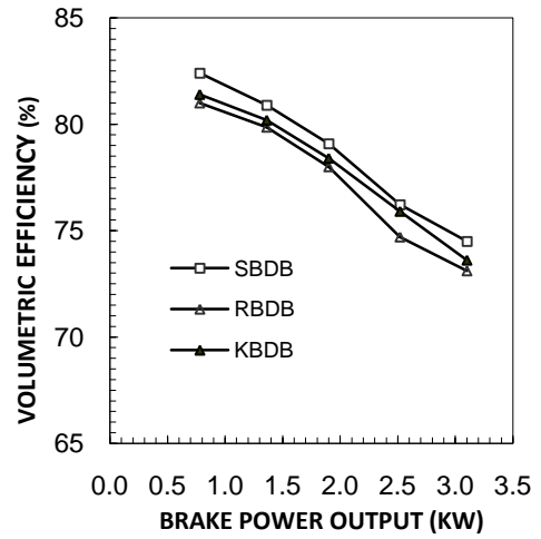
Figure 5. Comparison of volumetric efficiency with power output for different Biodiesel blends
