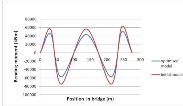
Fig 22: variation of bending moment along girder for optimized and initial models
