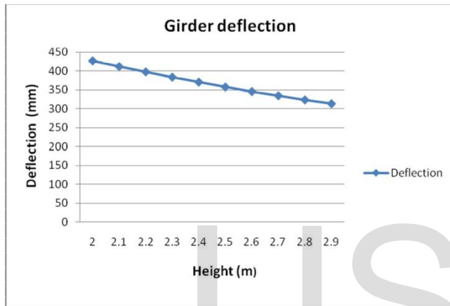
Fig 5: comparison of girder deflection and height of girder.
