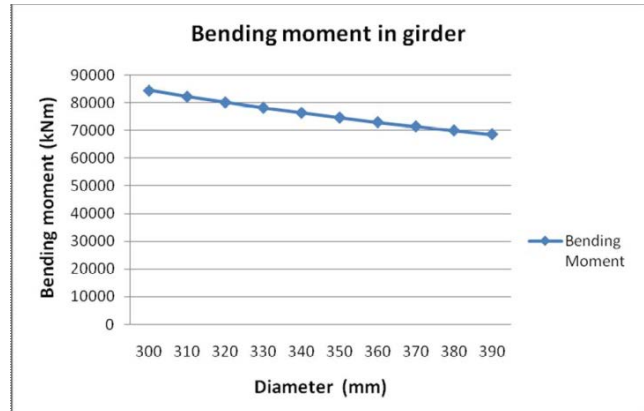
Fig 13: comparison of bending moment in girder and diameter of main cable.
