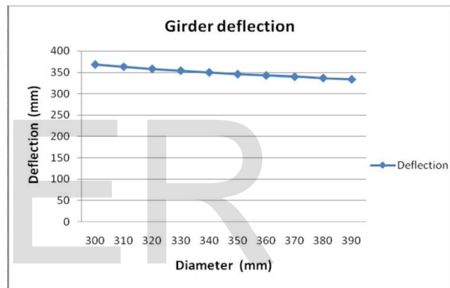
Fig 14: comparison of girder deflection and diameter of main cable.
