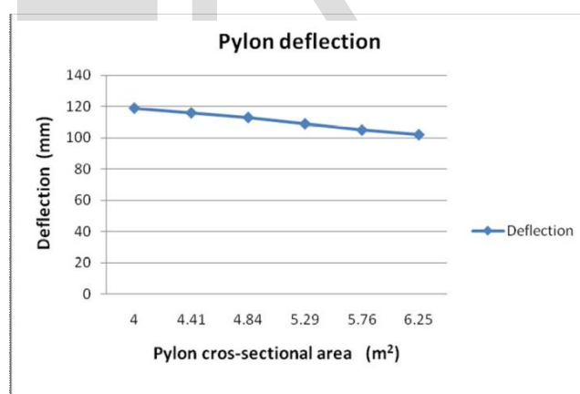
Fig 9: comparison of pylon deflection and area of pylon.
