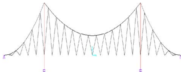
Fig 17: self anchored suspension bridge with inclined hangers
