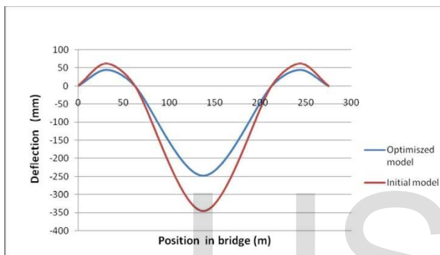
Fig 23: variation of deflection in girder for optimized and Initial models
