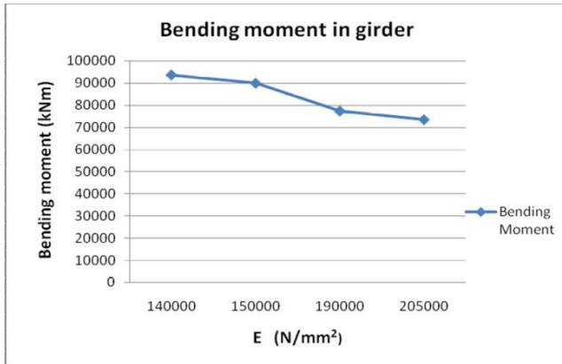
Fig 10: comparison of bending moment in girder and modulus of elasticity
