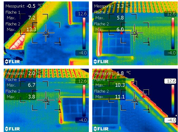
Fig. 11: Multi-image thermography
