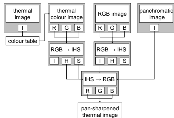
Fig. 12: Image data flow for thermal pan-sharpening
