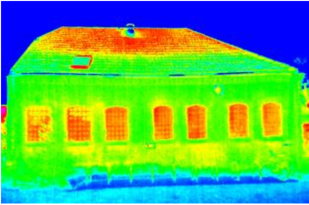
Fig. 13: Original thermal image
