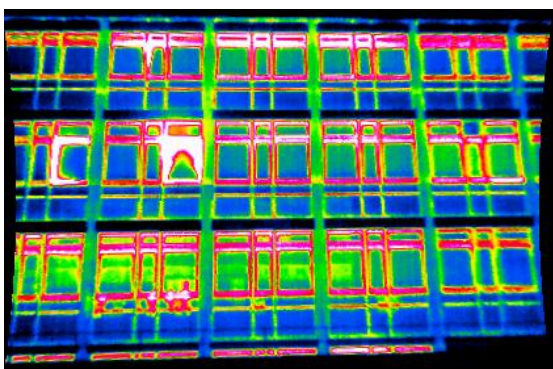
Fig. 10: Distortion-free thermal image
