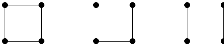
Figure 1: C_4 , P_4 and 2K_2
