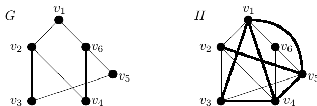
Figure 3: A partitioned 3-probe threshold graph (G, \mathcal{N}) where \mathcal{N} = \{\mathbb{N}_1, \mathbb{N}_2, \mathbb{N}_3\} , \mathbb{N}_1 = \{v_1, v_3, v_4\} , \mathbb{N}_2 = \{v_1, v_4, v_5\} , and \mathbb{N}_3 = \{v_2, v_5\} . H is a threshold embedding of G where the thin lines in H are those edges in G and those thick lines in H are new edges being added.
