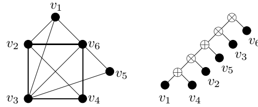
Figure 2: A threshold graph and its binary tree-decomposition where \otimes denotes a join-node and \oplus denotes a union-node.
